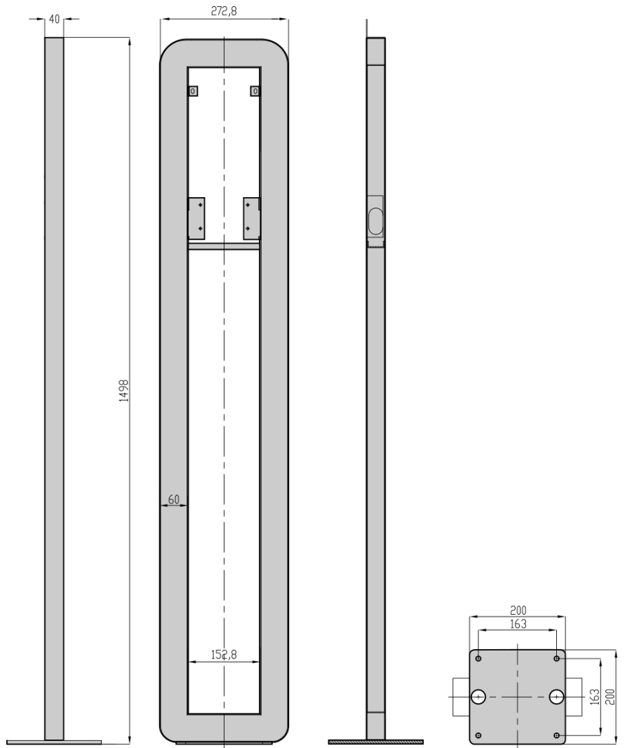
Figur 6: INCH monteringsstolpe
