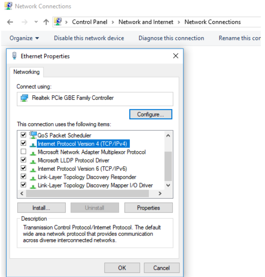
Figure 27: Locate Internet Protocol Version 4(TCP/IPv4) in network properties
