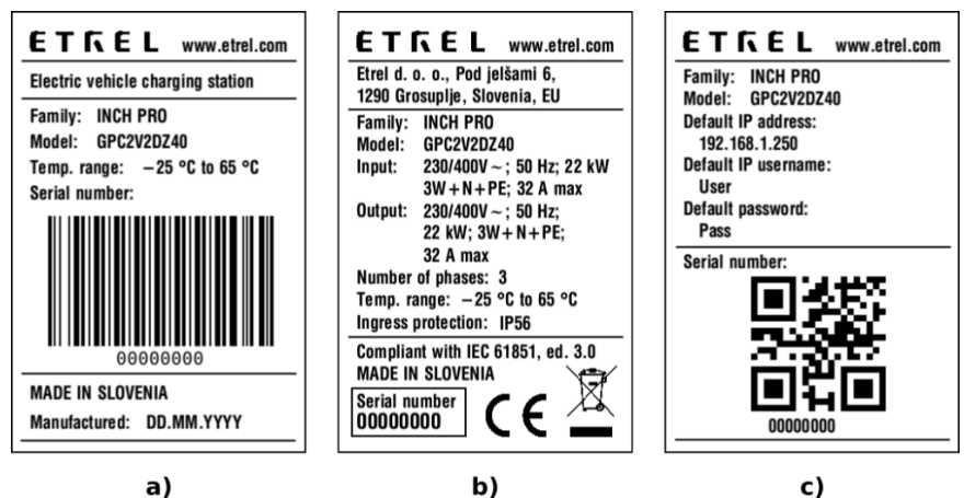
Figure 8: Three different stickers, sticker on the delivery package, on the maintenance doors and inside the maintenance space, behind maintenance doors
