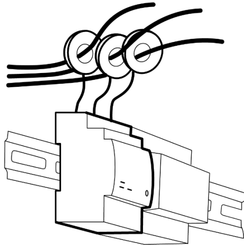
Figure 7: Load Guard
