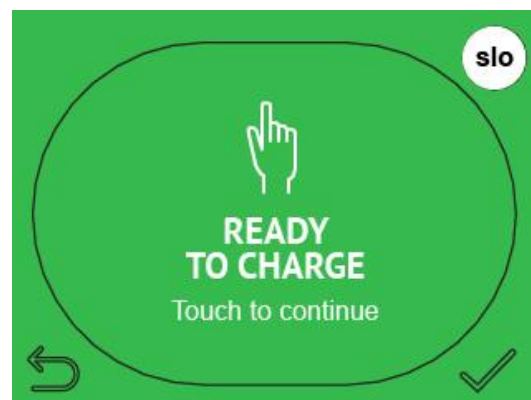
Figure 9: Screen saver
